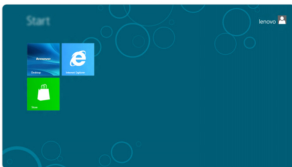
Start screen
