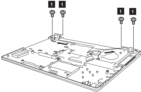
Figure 11. Removal steps of LCD unit and upper cover
