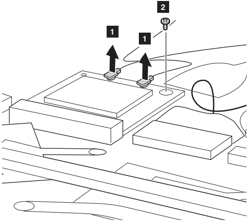
Figure 7. Removal steps of PCI Express Mini Card for wireless LAN/WAN Disconnect the two wireless LAN cables (black, white) 1 , and then remove the screws 2 .
