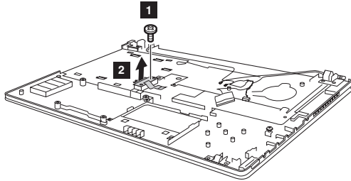
Figure 10. Removal steps of ODD transfer board
