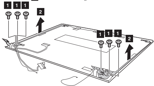
Figure 14. Removal steps of hinges
