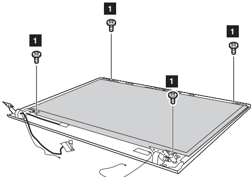
Figure 13. Removal steps of LCD panel
