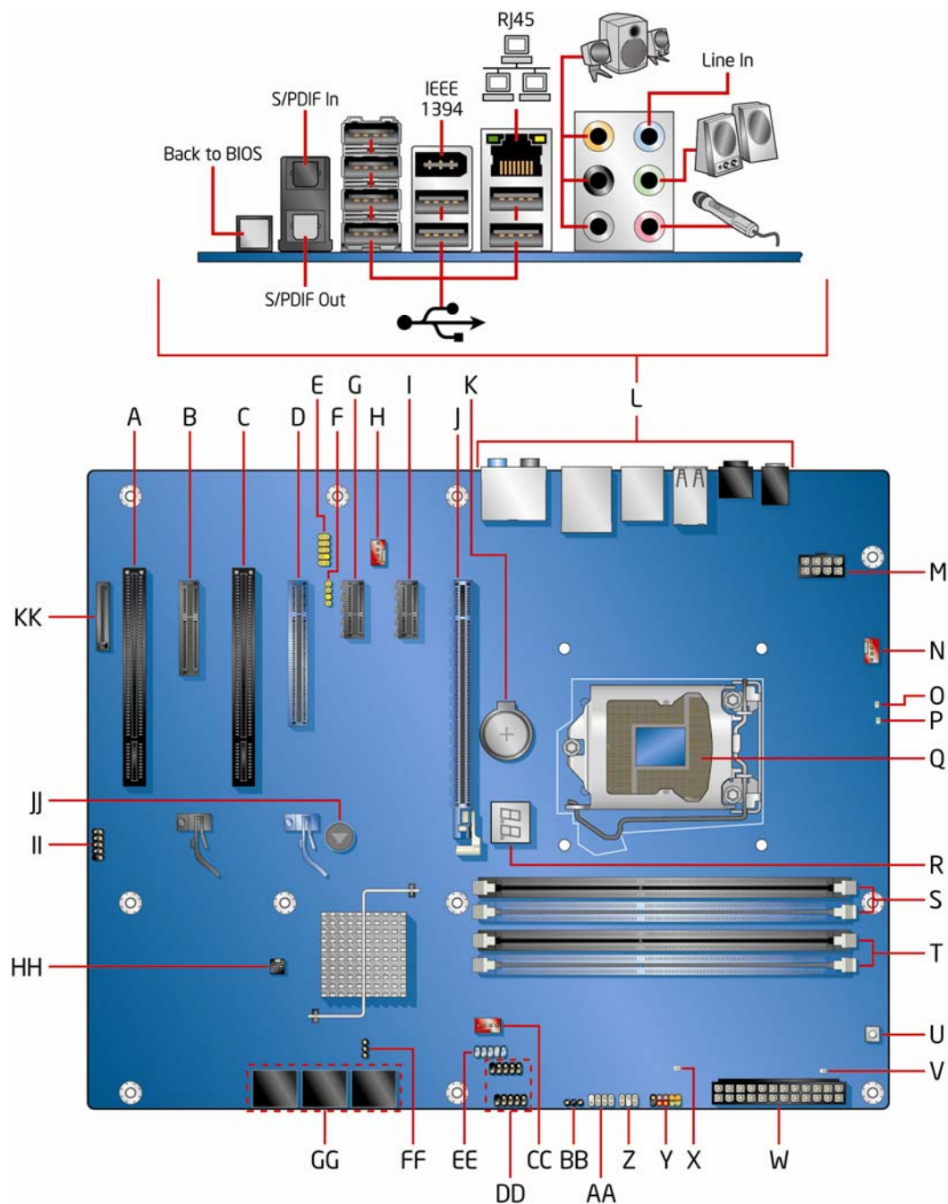
Figure 1. Intel Desktop Board DP55WG Components
