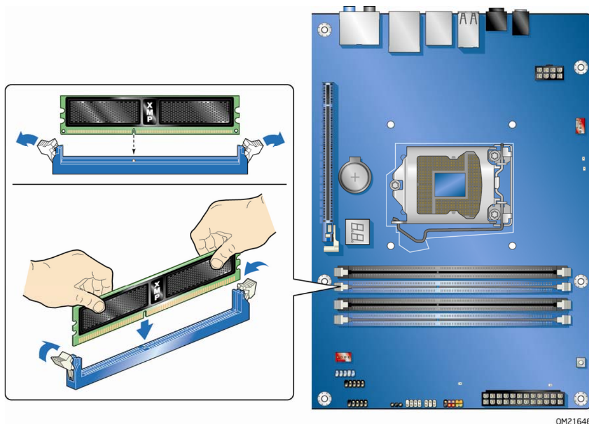
Figure 22. Installing a DIMM
