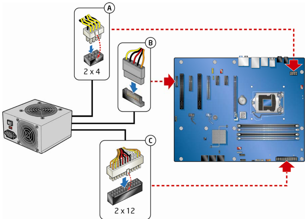
Figure 30. Connecting Power Supply Cables
