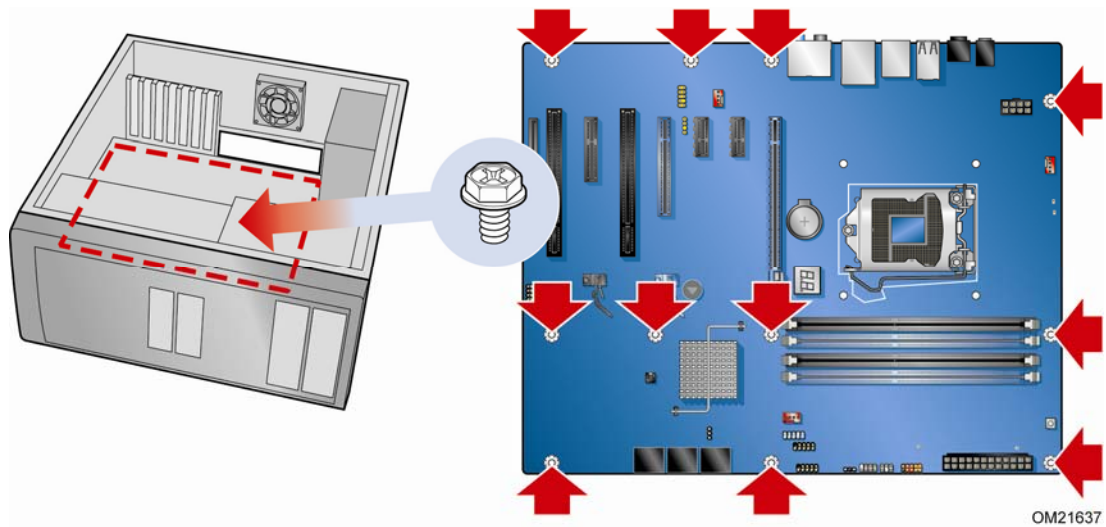
Figure 9. Intel Desktop Board DP55WG Mounting Screw Hole Locations
