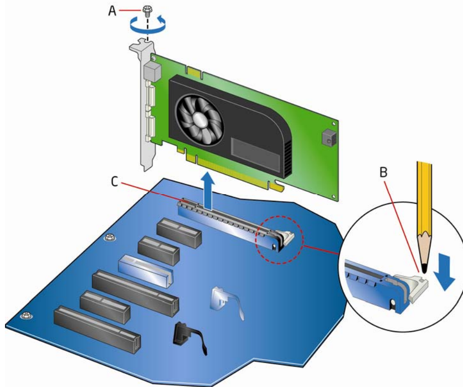
Figure 24. Removing a PCI Express x16 Graphics Card
