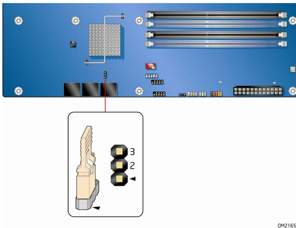
Figure 31. Location of the BIOS Configuration Jumper Block
