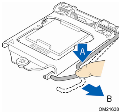
Figure 10. Unlatch the Socket Lever
