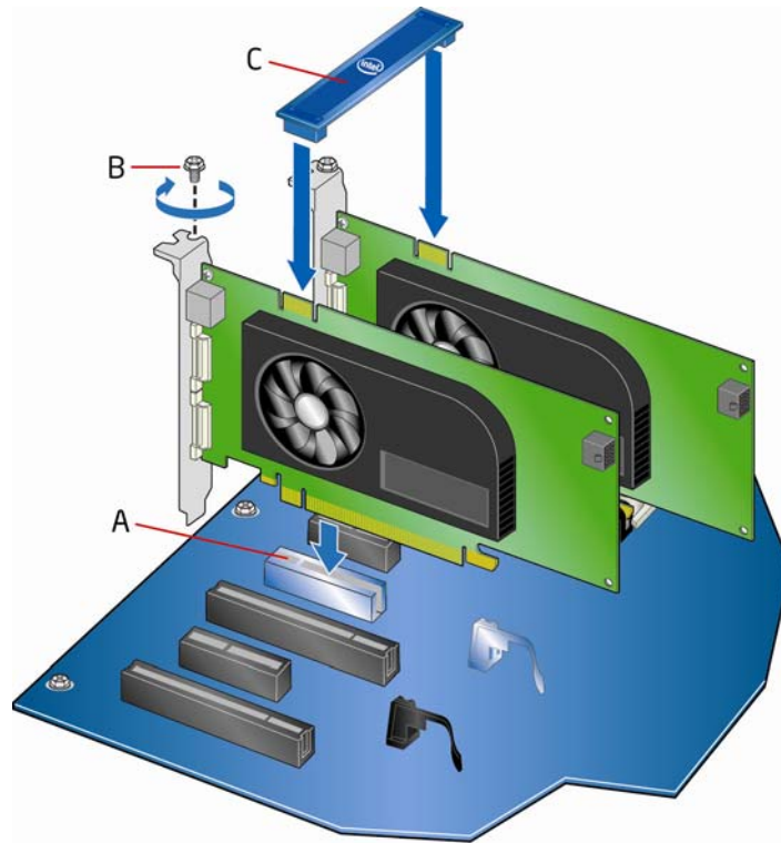
Figure 25. Installing Linked PCI Express Graphics Cards
