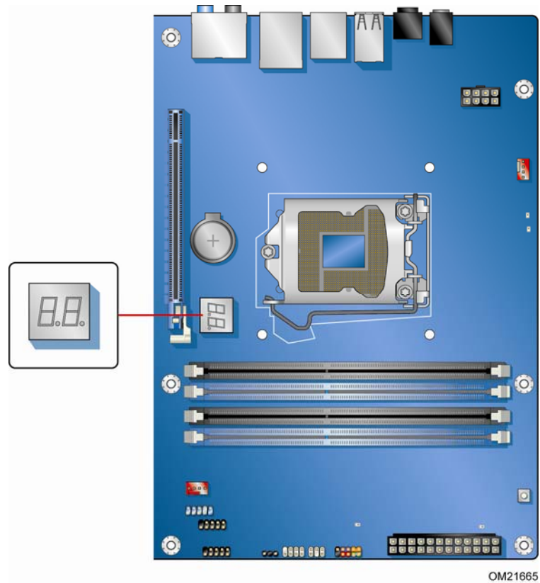
Figure 33. Location of the POST Code LED Display
