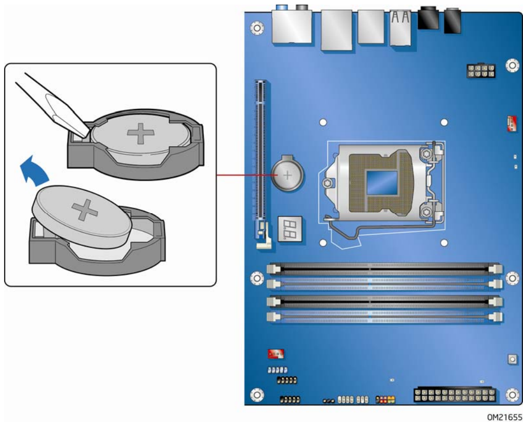
Figure 32. Removing the Battery
