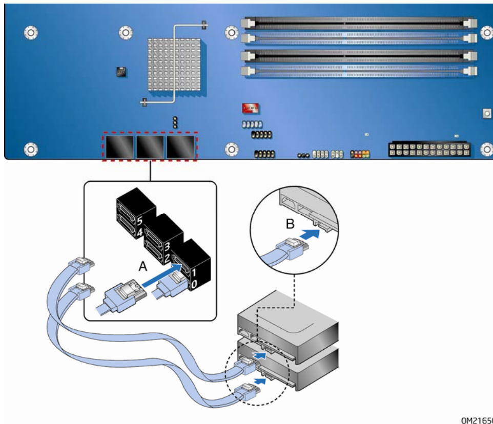
Figure 26. Connecting the Serial ATA Cables
