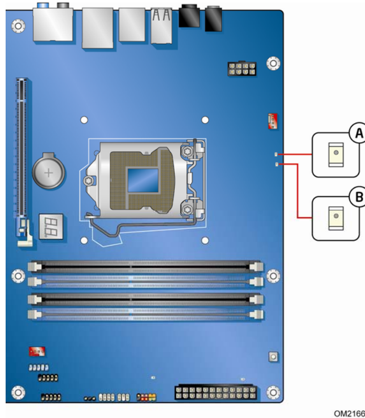
Figure 6. Location of the Processor and Voltage Regulator LEDs
