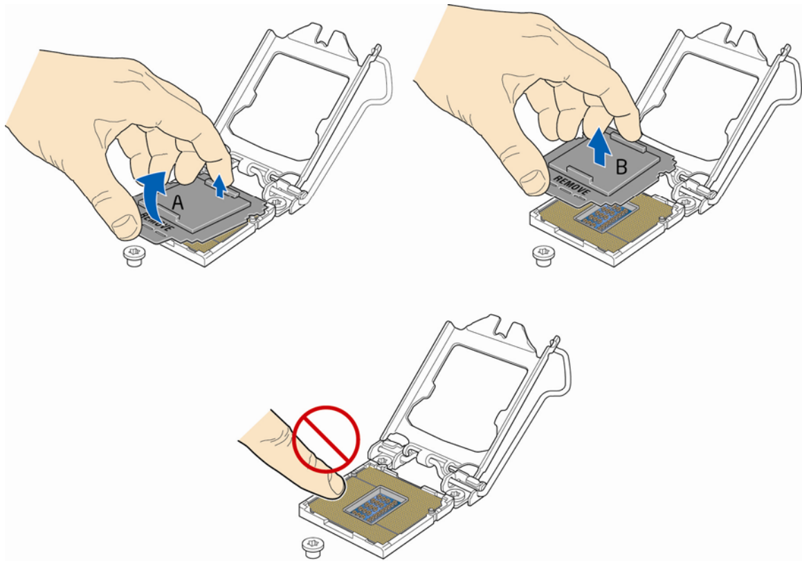
Figure 12. Remove the Socket Cover
