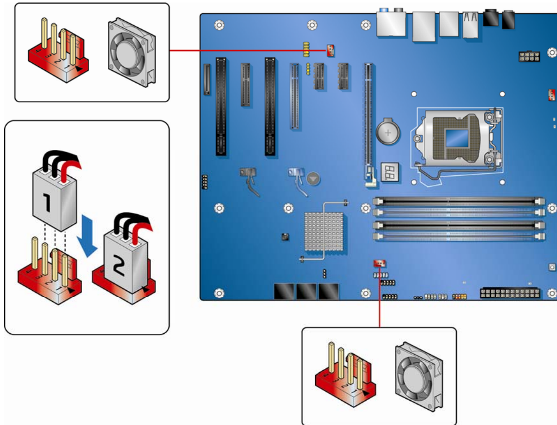
Figure 29. Location of the Chassis Fan Headers
