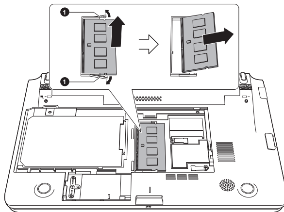
Figure 3-10 Removing the memory module
