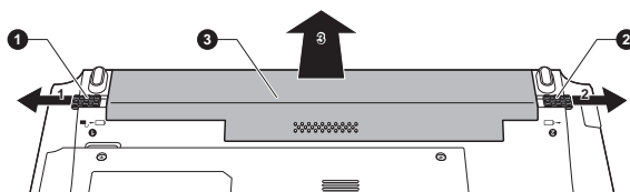
Figure 5-1 Releasing the battery pack
