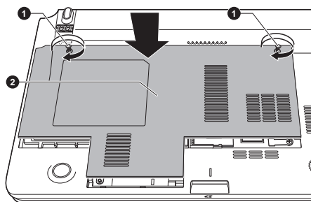
Figure 3-13 Seating the memory module cover
