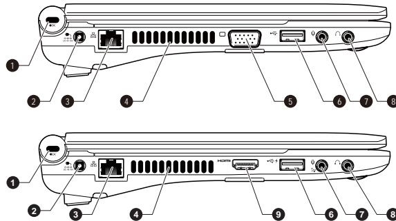
Figure 2-2 The left side of the computer
